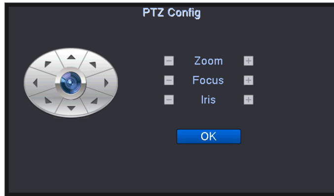
Patrol setting
