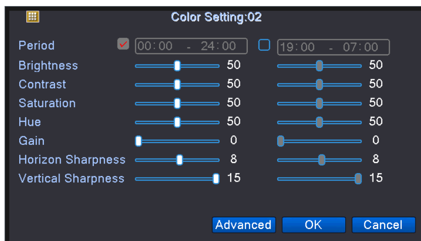
Color Setting
