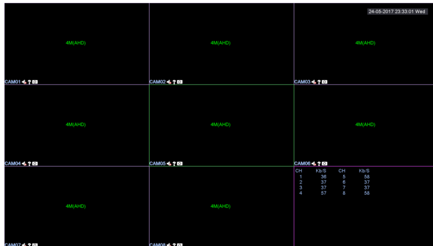
Preview status
